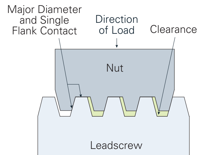
Radial Load on a General Purpose Nut
