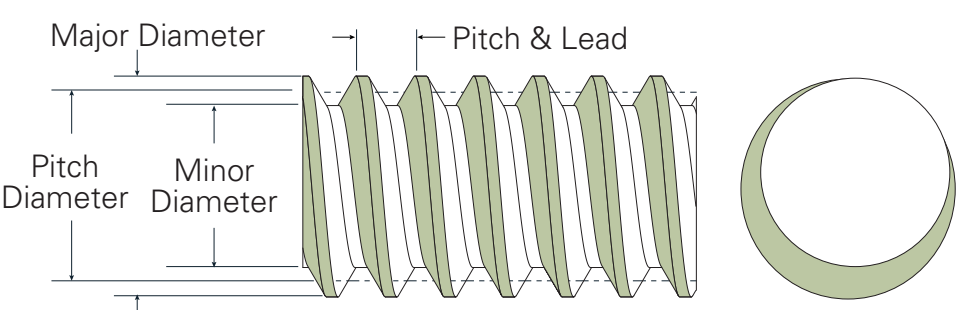
Single Start
