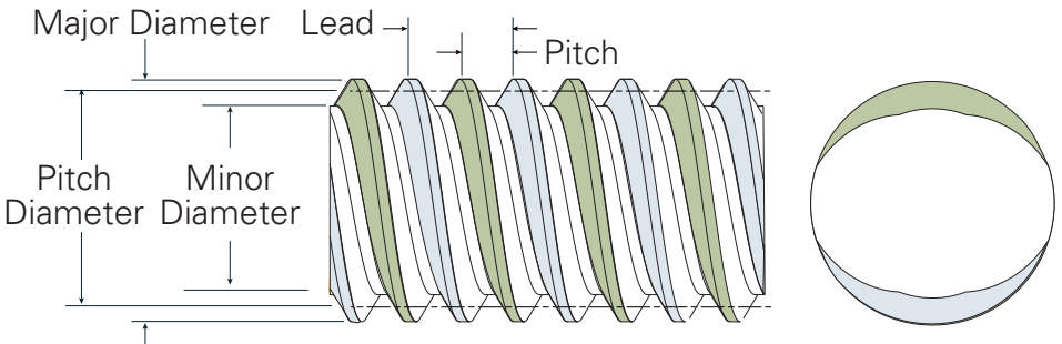
Double Start
