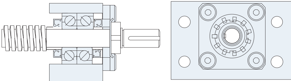
Universal Double Bearing Mount Fixed
