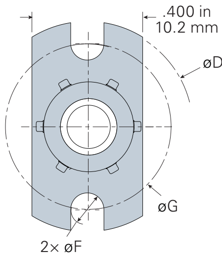
Two-Hole Flange Diameter Ranges: .078 – .188 in 2.0 – 5.0 mm
