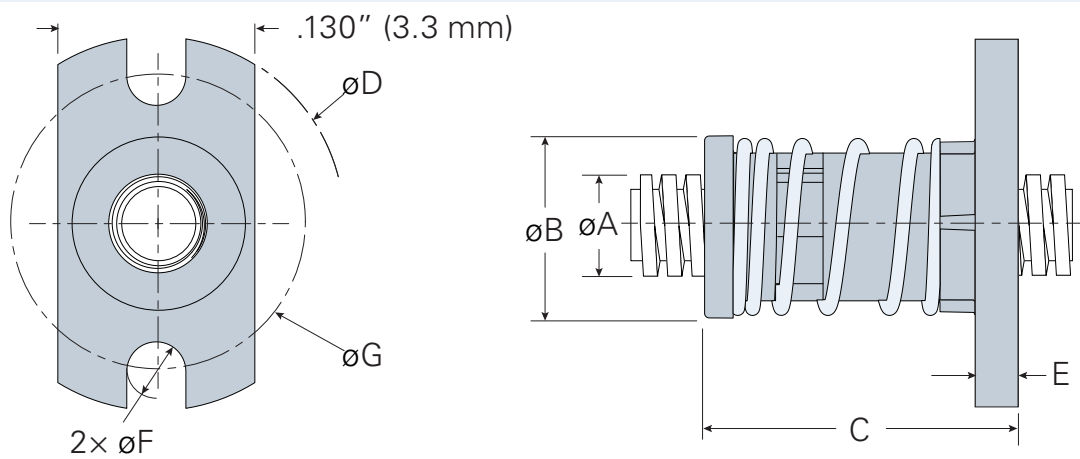
Two-Hole Flange Diameter Ranges: .078 – .188 in 2.0 – 5.0 mm
