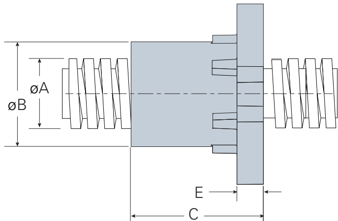
Three-Hole Flange Diameter Ranges:. 195 – 1.000 in 5.5 – 25.4 mm
